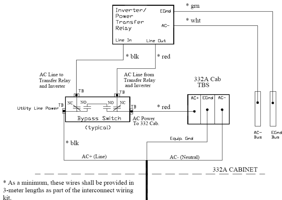
FIGURE 1 – UPS UTILITY POWER CONNECTION DIAGRAM
